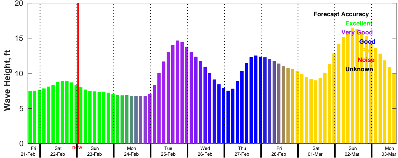
CMEMS Wave Forecast for NDBC 46028 from 21-Feb-2025 16:00:00 to 03-Mar-2025 16:00:00
