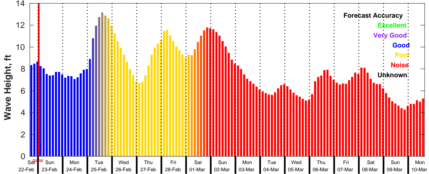
GFS Wave Forecast for NDBC 46028 from 22-Feb-2025 16:00:00 to 10-Mar-2025 16:00:00
