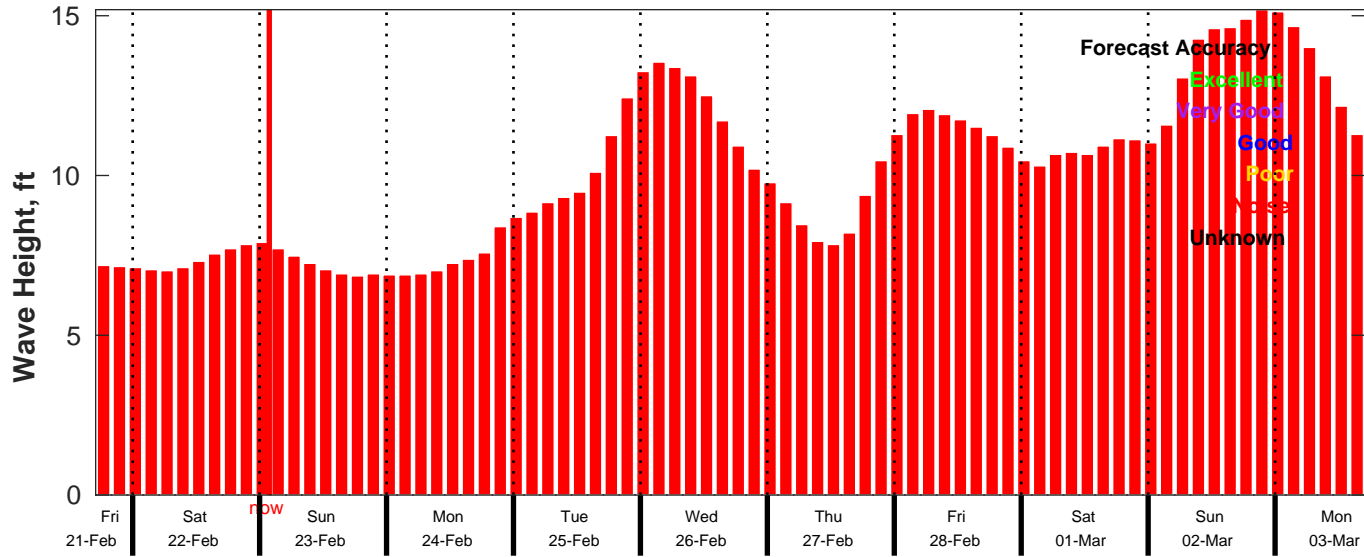
CMEMS Wave Forecast for NDBC 46053 from 21-Feb-2025 17:00:00 to 03-Mar-2025 17:00:00
