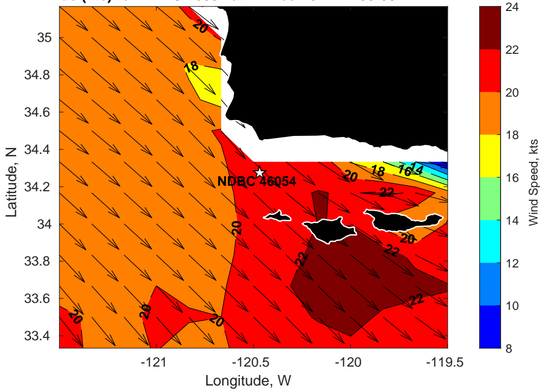
Winds (kts) for NDBC 46054 at 12-Dec-2024 21:00:00
