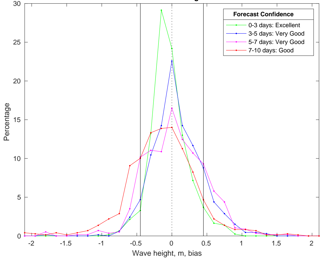
NDBC 46054 vs CMEMS Waves Bias Histogram: 23-Feb-2025
