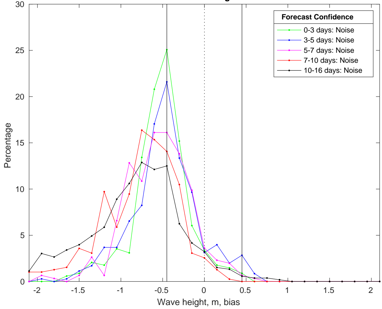
NDBC 46054 vs GFS Waves Bias Histogram: 23-Feb-2025
