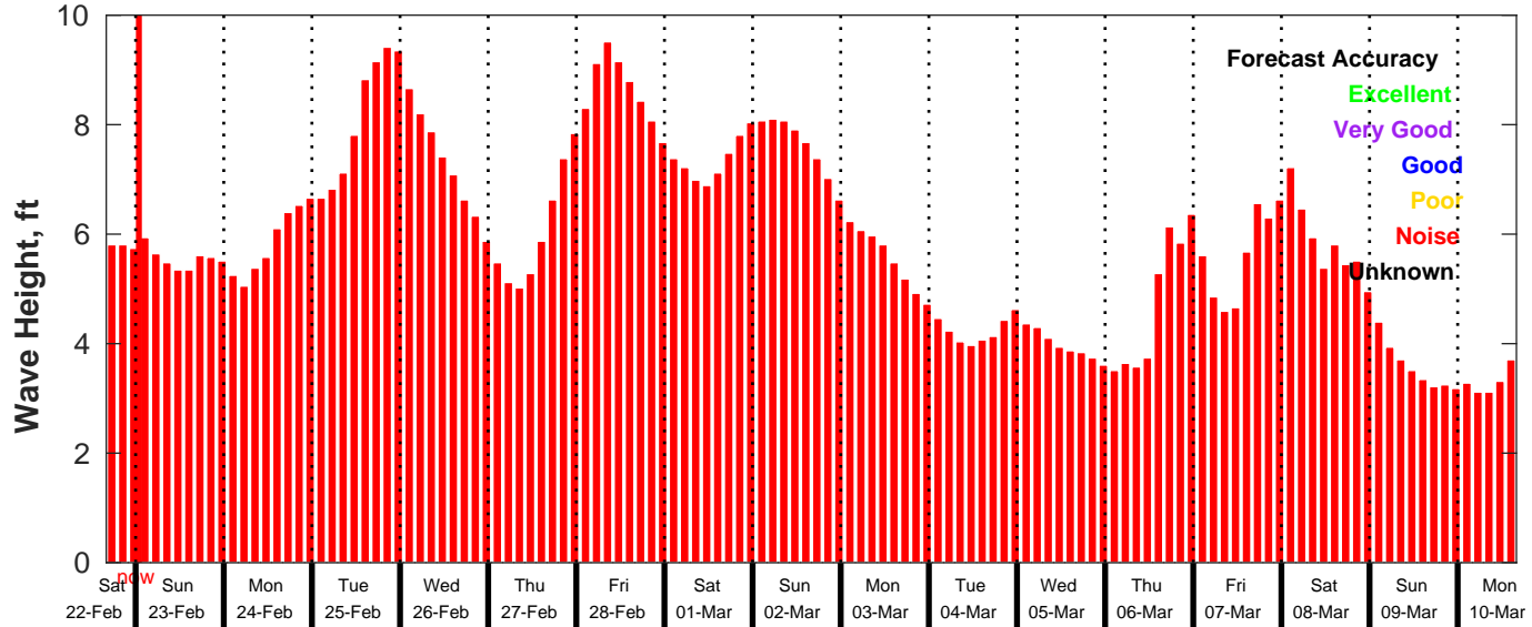
GFS Wave Forecast for NDBC 46054 from 22-Feb-2025 16:00:00 to 10-Mar-2025 16:00:00
