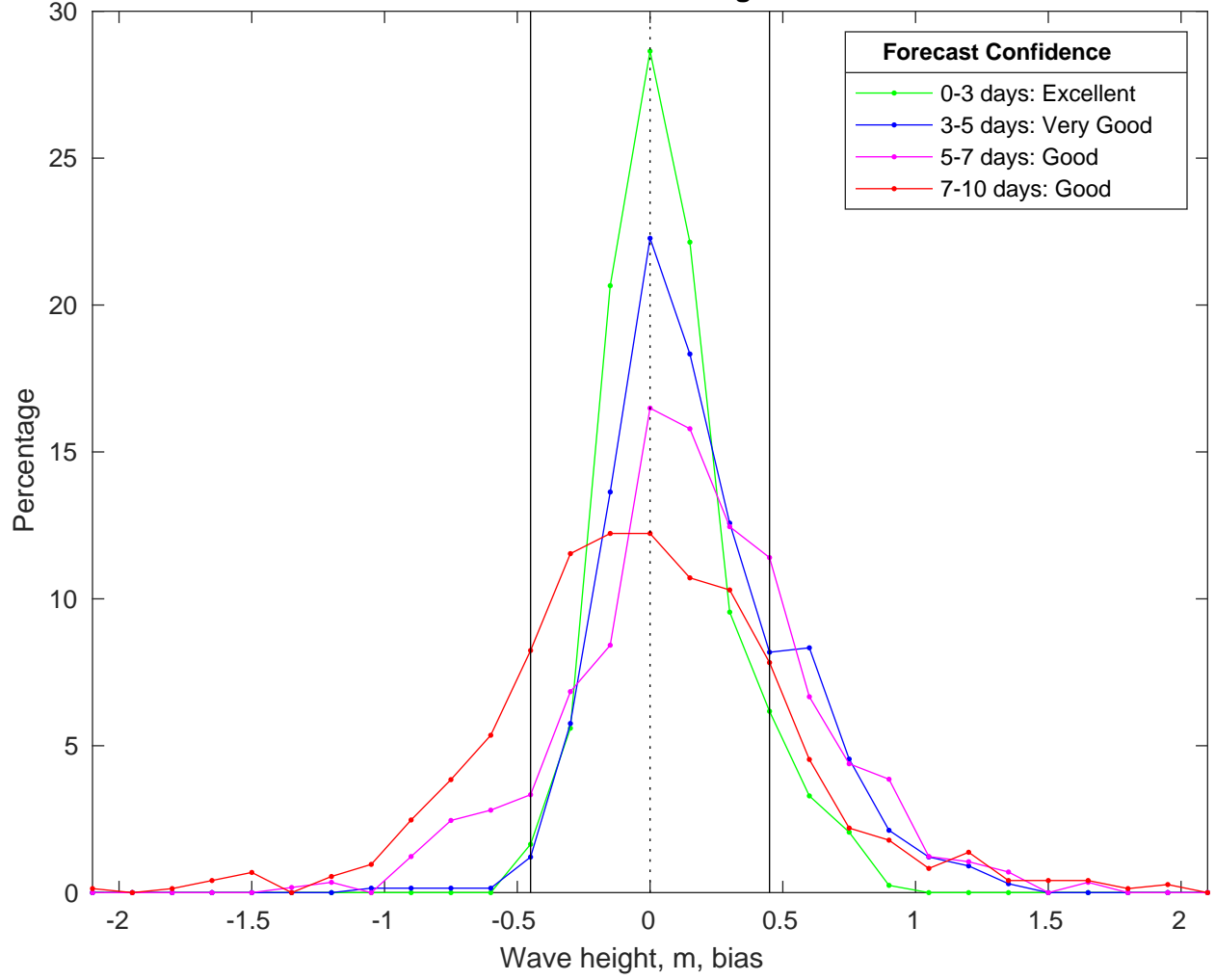
NDBC 46069 vs CMEMS Waves Bias Histogram: 23-Feb-2025
