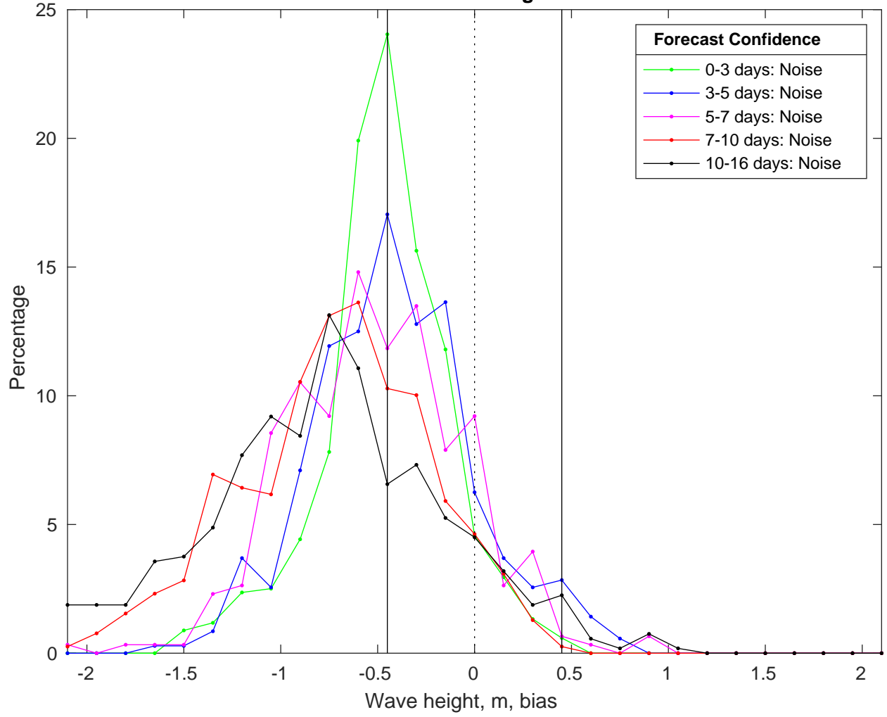
NDBC 46069 vs GFS Waves Bias Histogram: 23-Feb-2025
