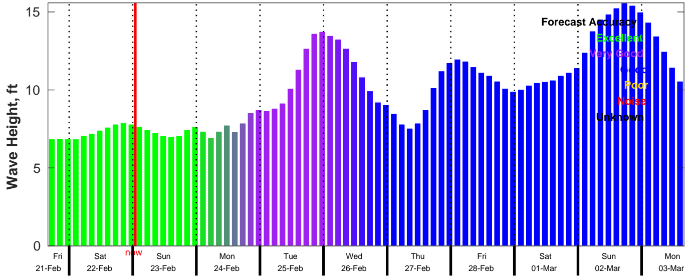
CMEMS Wave Forecast for NDBC 46069 from 21-Feb-2025 16:00:00 to 03-Mar-2025 16:00:00
