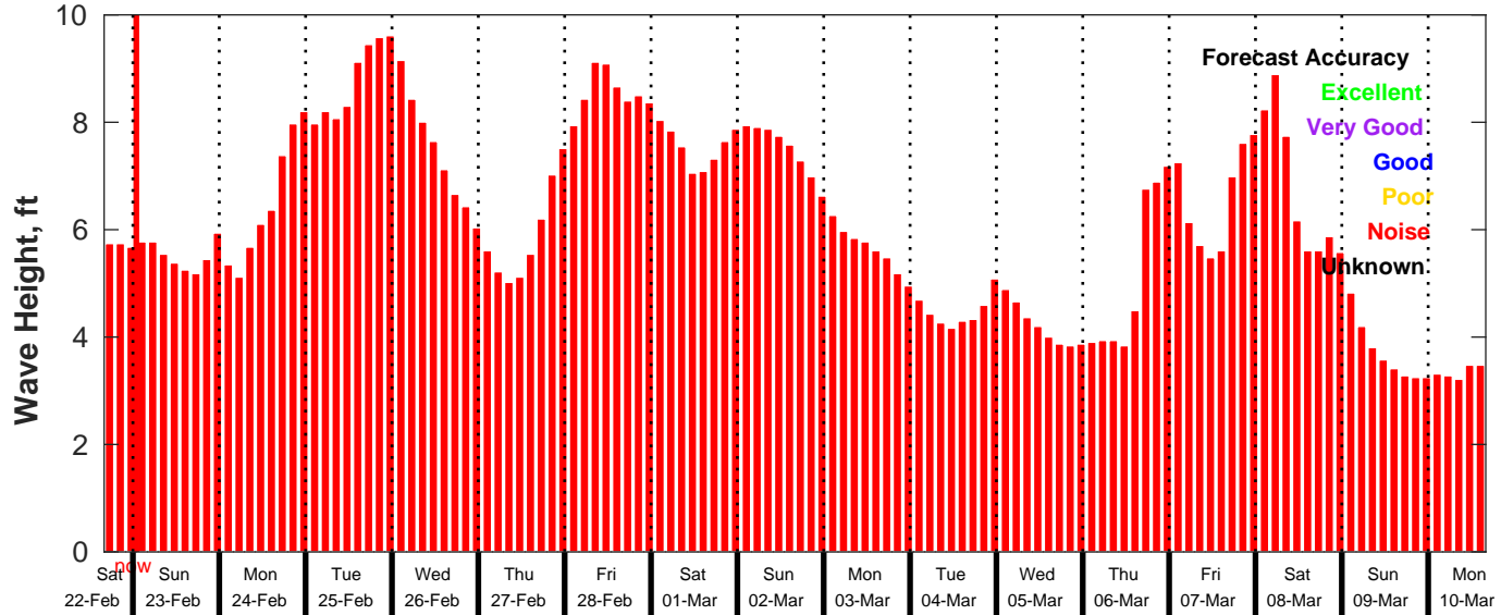
GFS Wave Forecast for NDBC 46069 from 22-Feb-2025 16:00:00 to 10-Mar-2025 16:00:00
