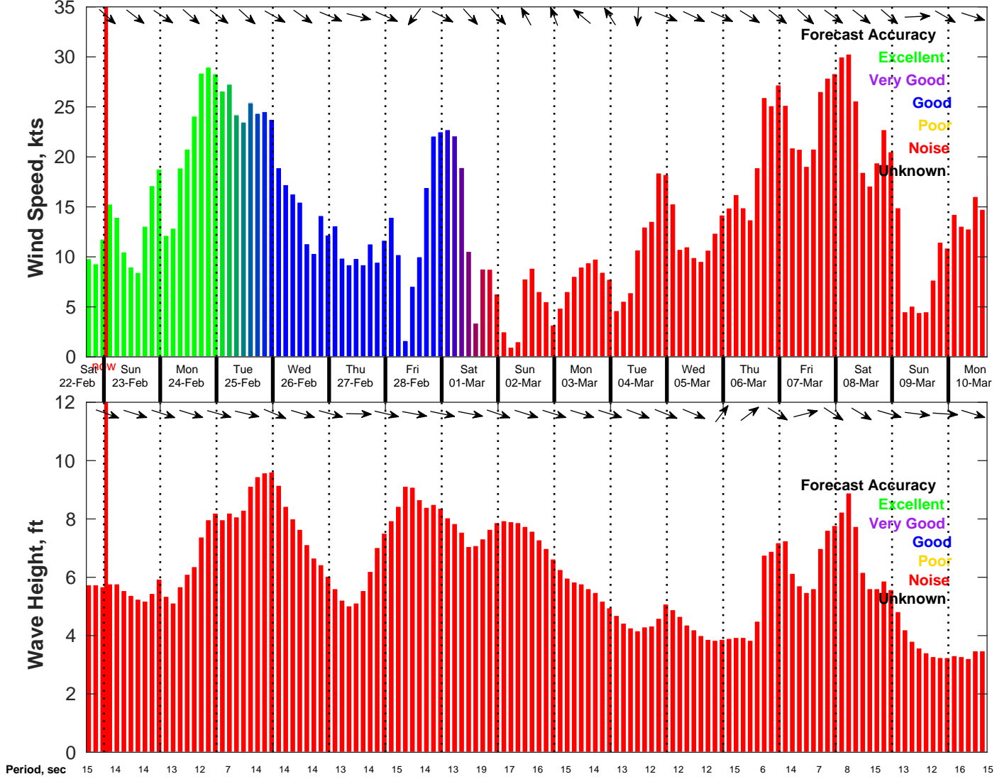
Wind & Wave Forecast for NDBC 46069 from 22-Feb-2025 16:00:00 to 10-Mar-2025 16:00:00
