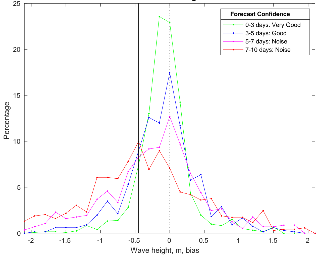
NDBC 46246 vs CMEMS Waves Bias Histogram: 23-Feb-2025
