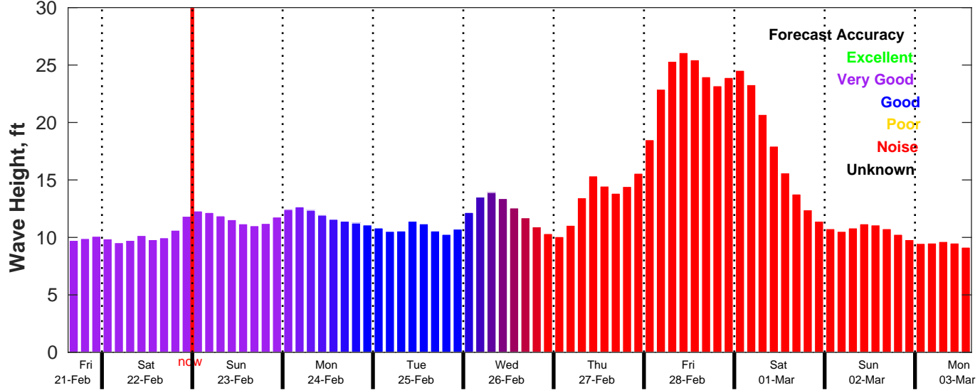
CMEMS Wave Forecast for NDBC 46246 from 21-Feb-2025 15:00:00 to 03-Mar-2025 15:00:00
