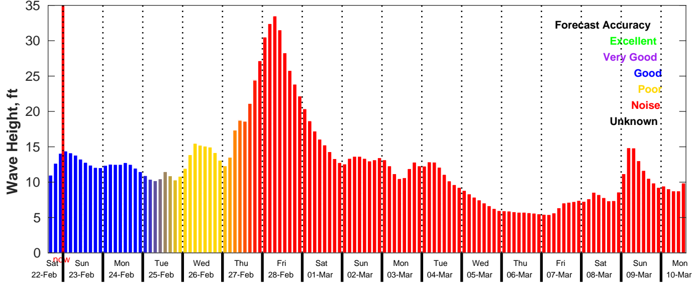
GFS Wave Forecast for NDBC 46246 from 22-Feb-2025 15:00:00 to 10-Mar-2025 15:00:00
