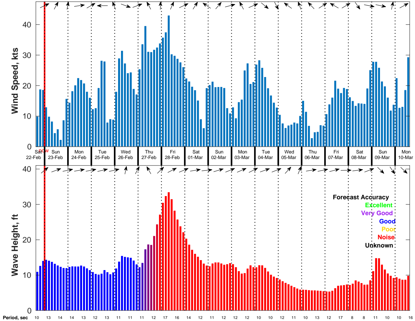
Wind & Wave Forecast for NDBC 46246 from 22-Feb-2025 15:00:00 to 10-Mar-2025 15:00:00
