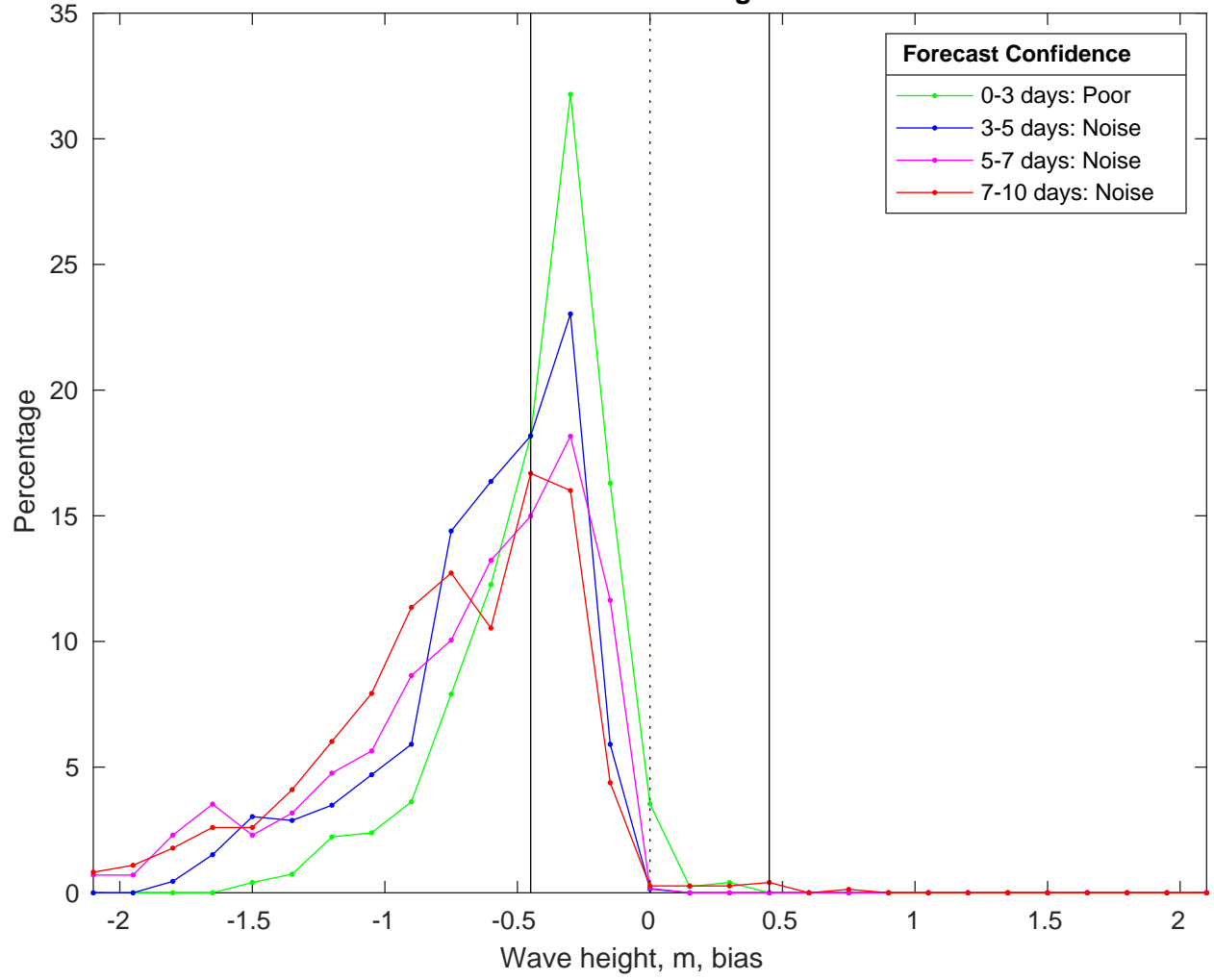
NDBC 51209 vs CMEMS Waves Bias Histogram: 23-Feb-2025
