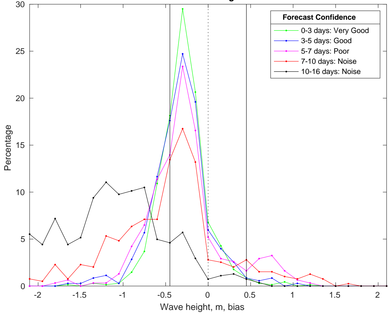
NDBC 51209 vs GFS Waves Bias Histogram: 23-Feb-2025
