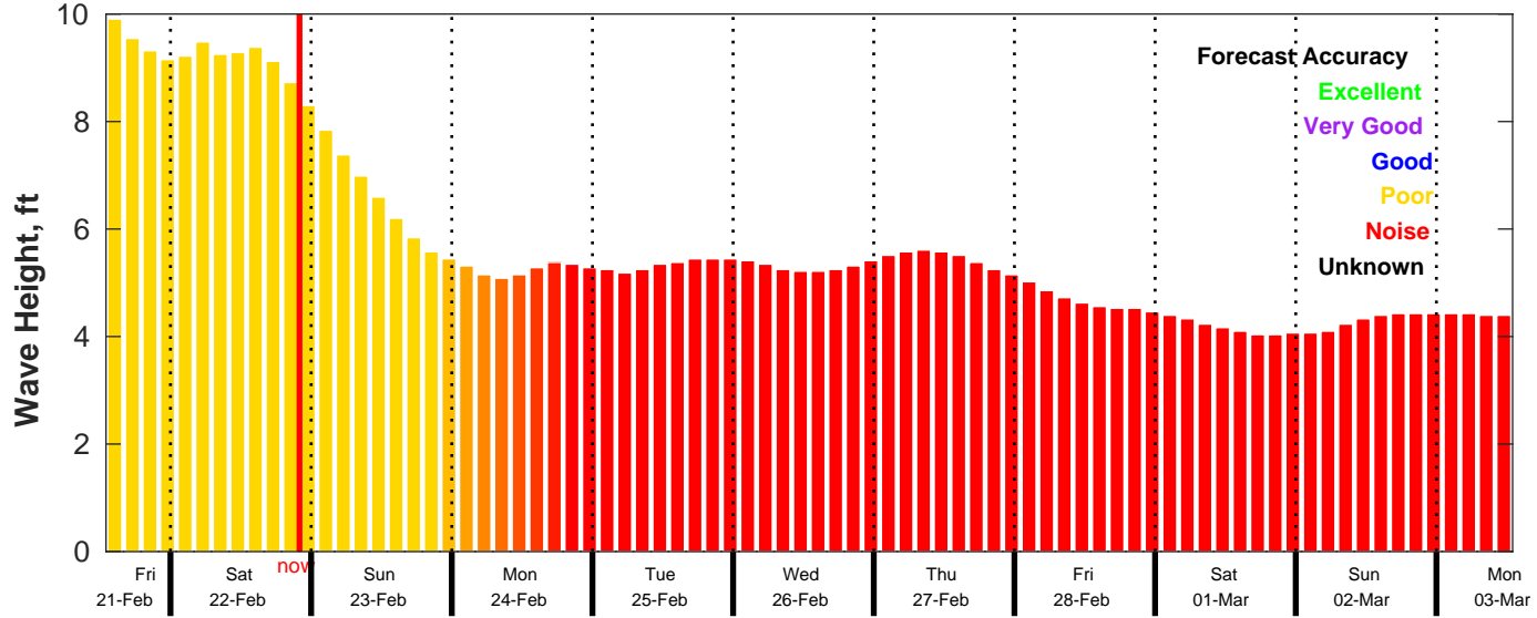
CMEMS Wave Forecast for NDBC 51209 from 21-Feb-2025 13:00:00 to 03-Mar-2025 13:00:00
