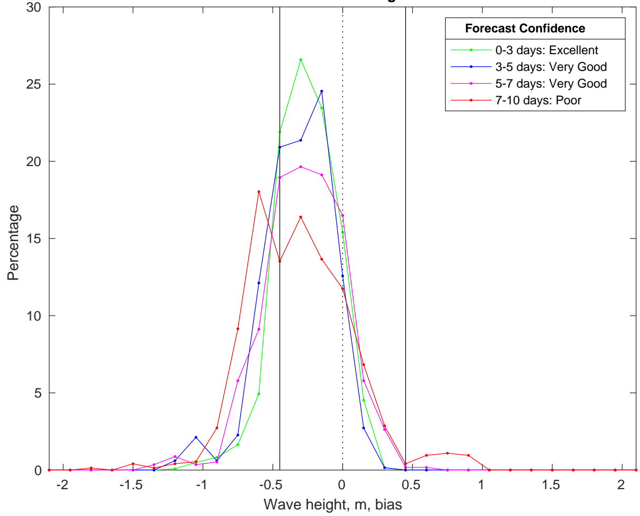
NDBC 52211 vs CMEMS Waves Bias Histogram: 23-Feb-2025
