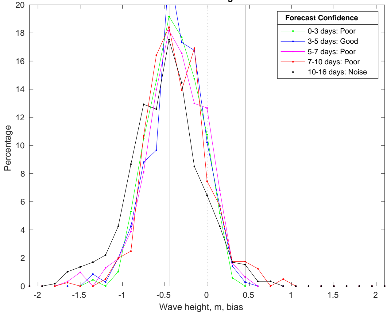
NDBC 52211 vs GFS Waves Bias Histogram: 23-Feb-2025
