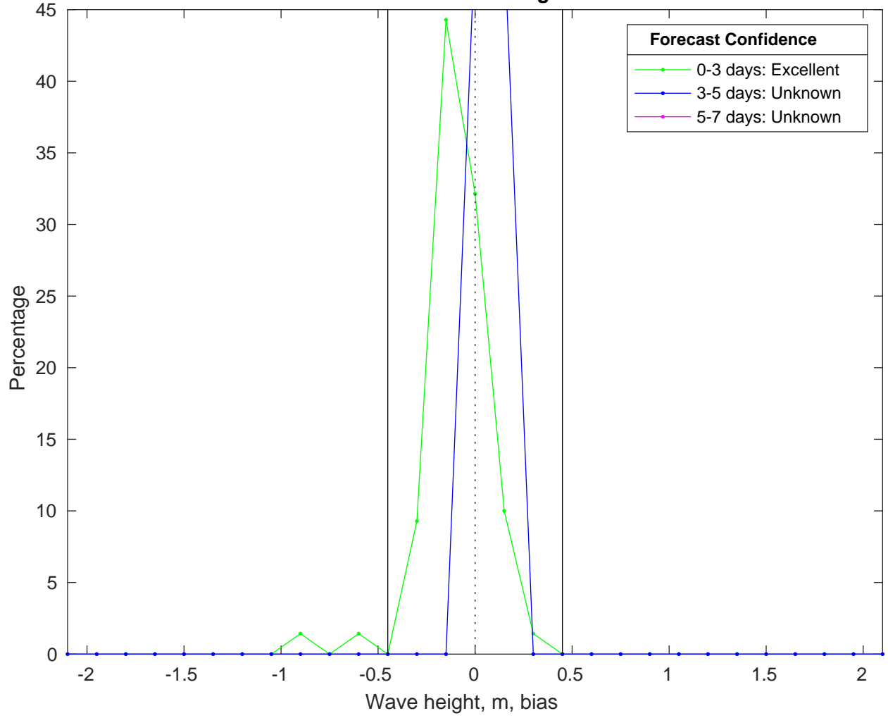
NDBC 52212 vs CMEMS Waves Bias Histogram: 23-Feb-2025
