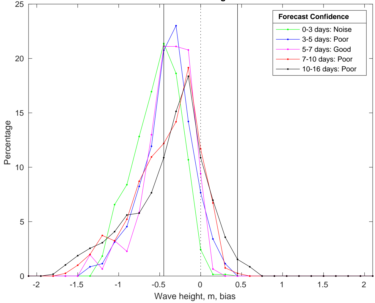
NDBC 52213 vs GFS Waves Bias Histogram: 23-Feb-2025
