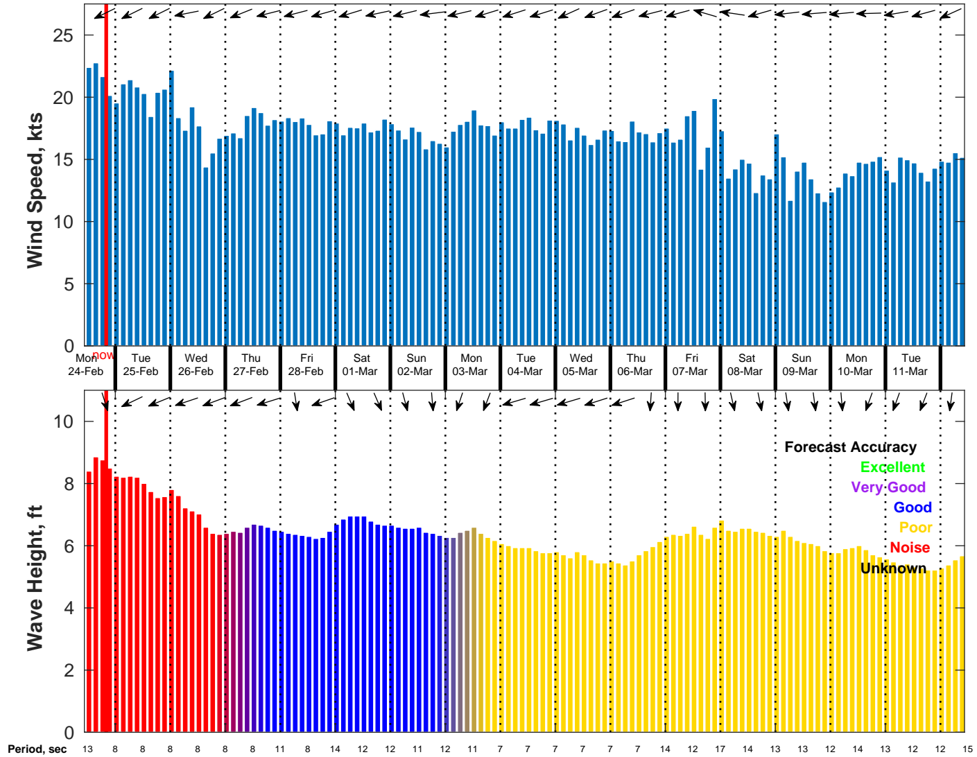
Wind & Wave Forecast for NDBC 52213 from 23-Feb-2025 11:00:00 to 11-Mar-2025 11:00:00
