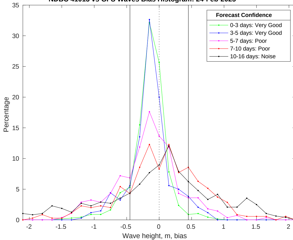
NDBC 41013 vs GFS Waves Bias Histogram: 24-Feb-2025
