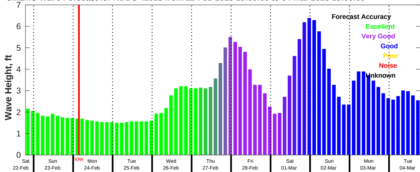
CMEMS Wave Forecast for NDBC 41013 from 22-Feb-2025 19:00:00 to 04-Mar-2025 19:00:00
