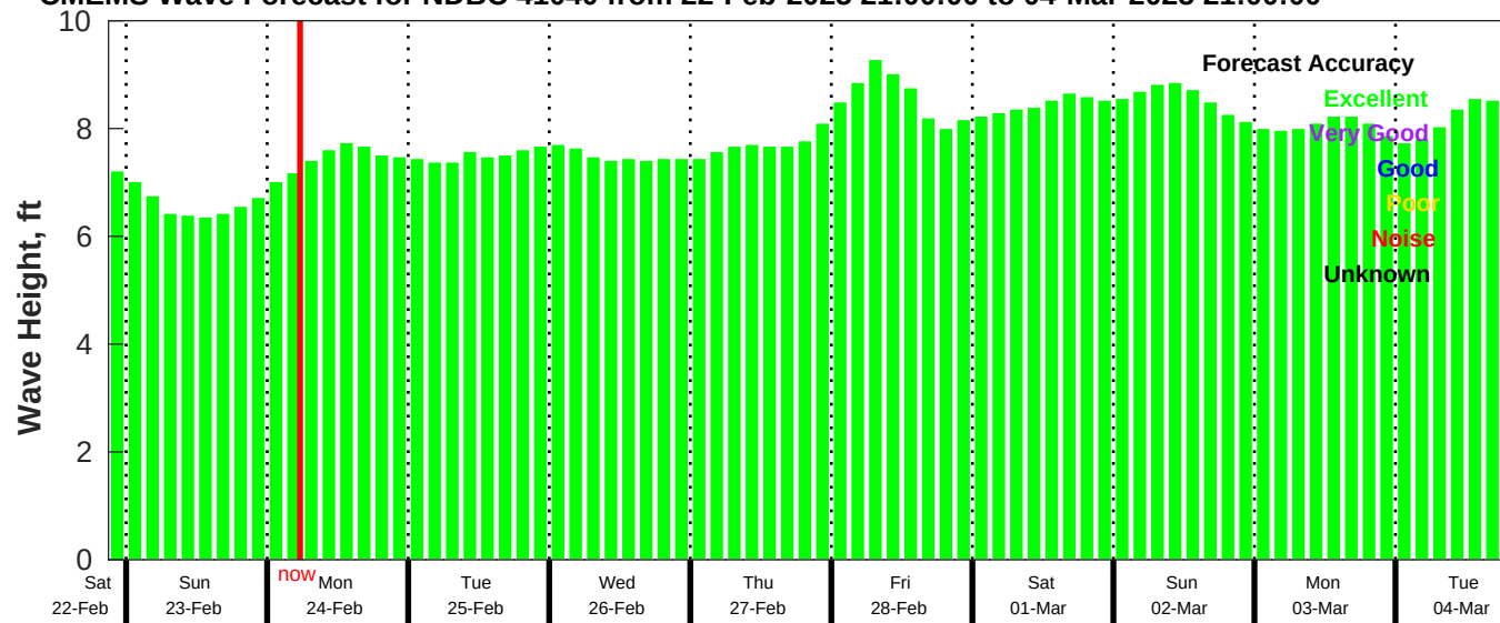
CMEMS Wave Forecast for NDBC 41040 from 22-Feb-2025 21:00:00 to 04-Mar-2025 21:00:00
