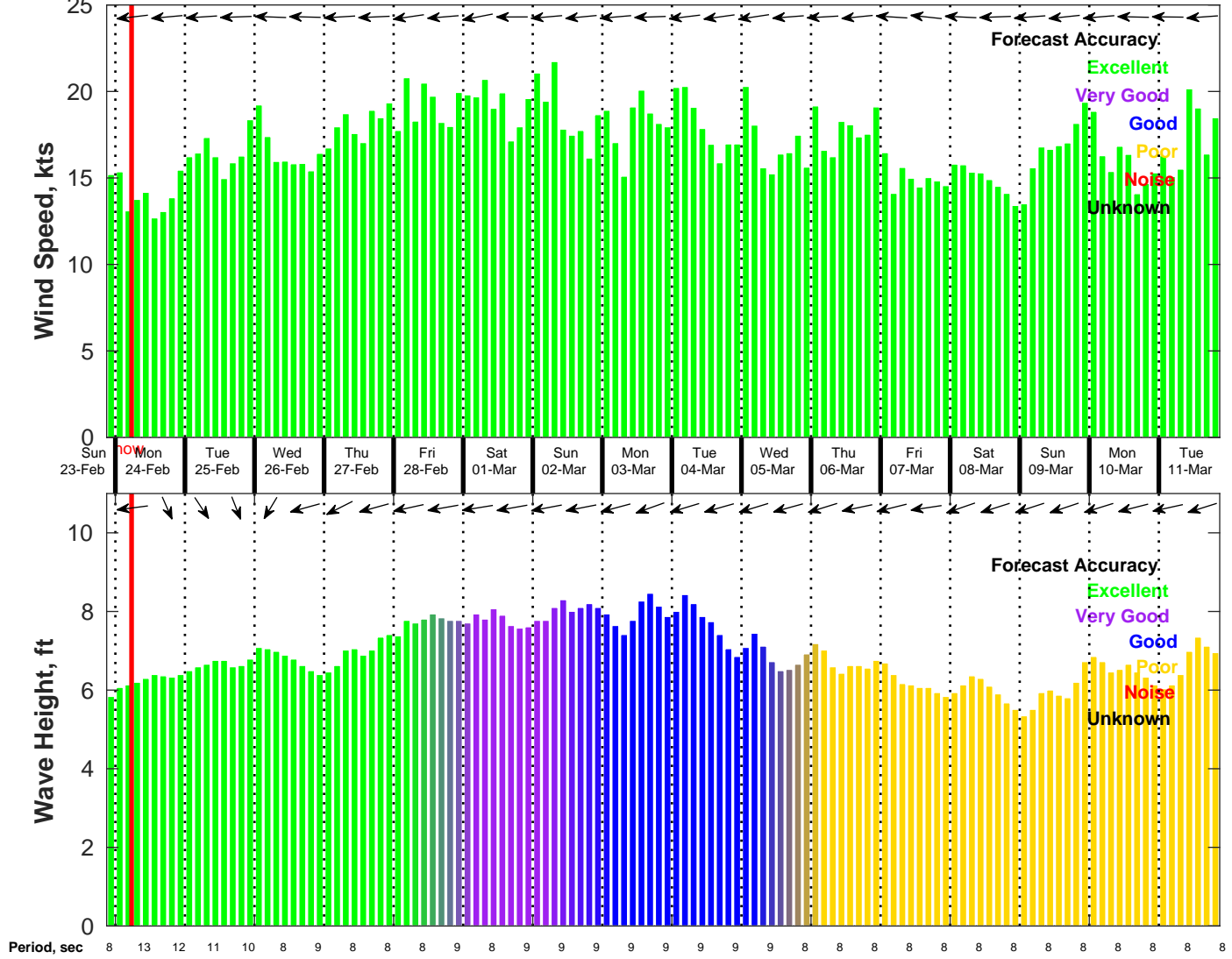
Wind & Wave Forecast for NDBC 41040 from 23-Feb-2025 21:00:00 to 11-Mar-2025 21:00:00
