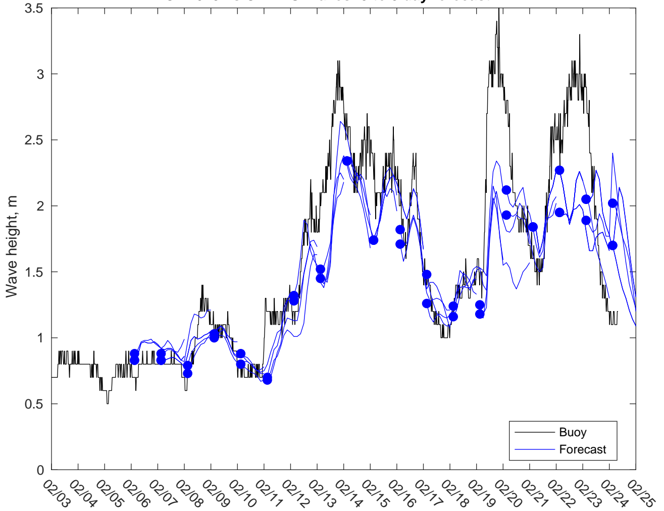
NDBC 42019 vs CMEMS Waves: 3 to 5 day forecast
