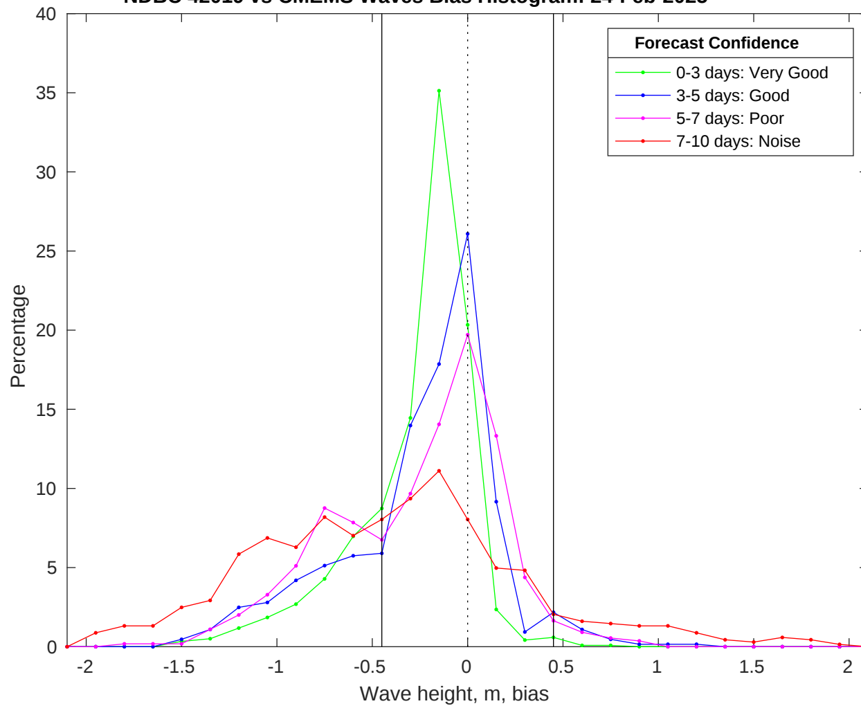
NDBC 42019 vs CMEMS Waves Bias Histogram: 24-Feb-2025
