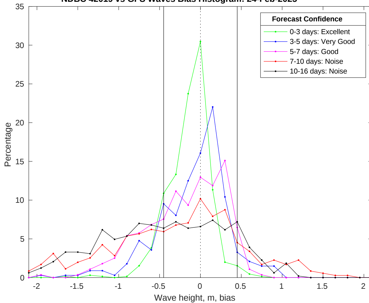
NDBC 42019 vs GFS Waves Bias Histogram: 24-Feb-2025
