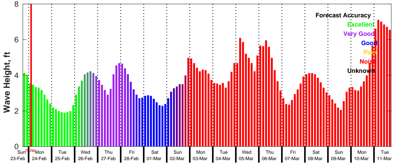
GFS Wave Forecast for NDBC 42019 from 23-Feb-2025 18:00:00 to 11-Mar-2025 18:00:00
