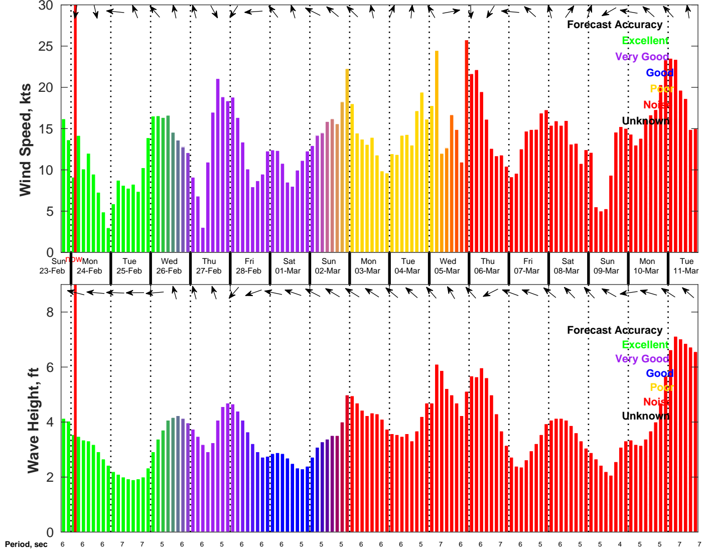
Wind & Wave Forecast for NDBC 42019 from 23-Feb-2025 18:00:00 to 11-Mar-2025 18:00:00
