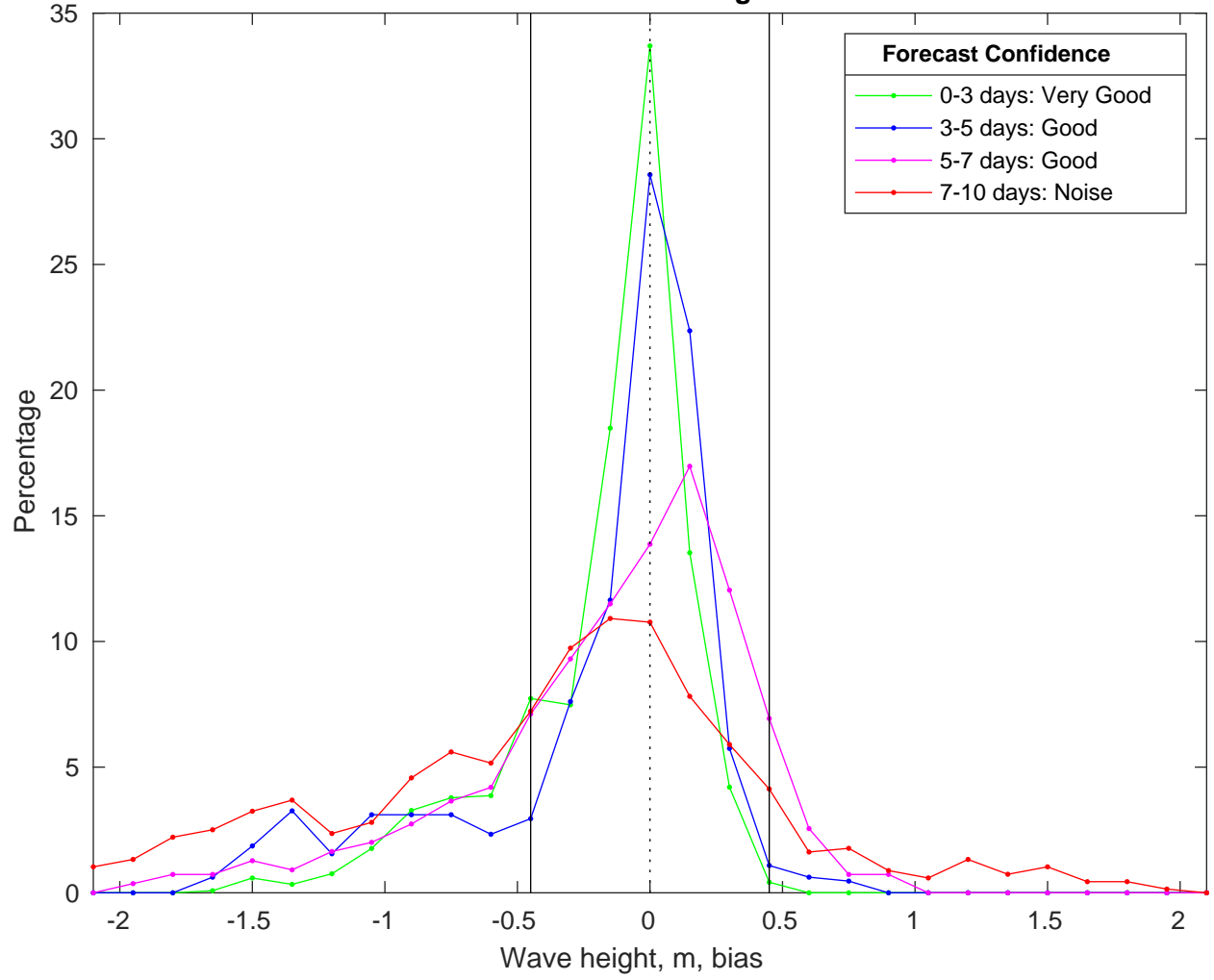
NDBC 42020 vs CMEMS Waves Bias Histogram: 24-Feb-2025
