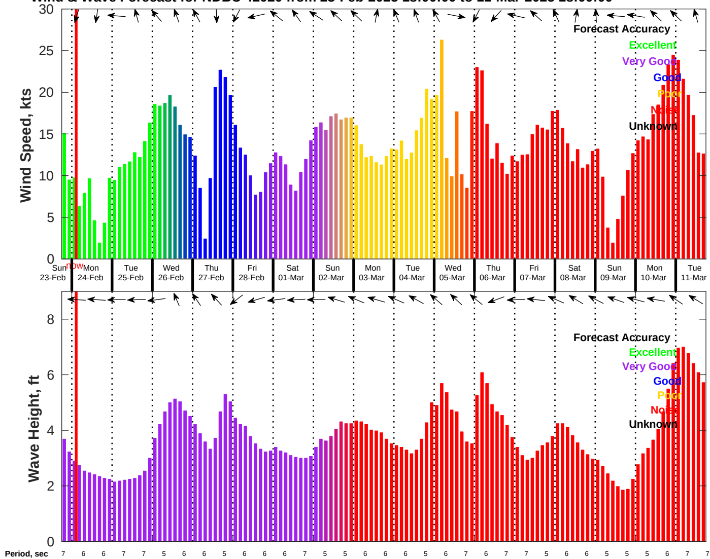
Wind & Wave Forecast for NDBC 42020 from 23-Feb-2025 18:00:00 to 11-Mar-2025 18:00:00
