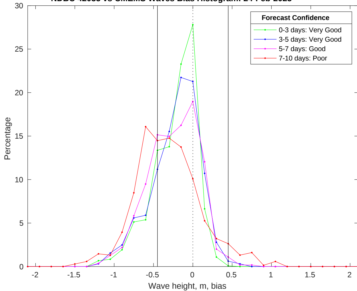
NDBC 42035 vs CMEMS Waves Bias Histogram: 24-Feb-2025
