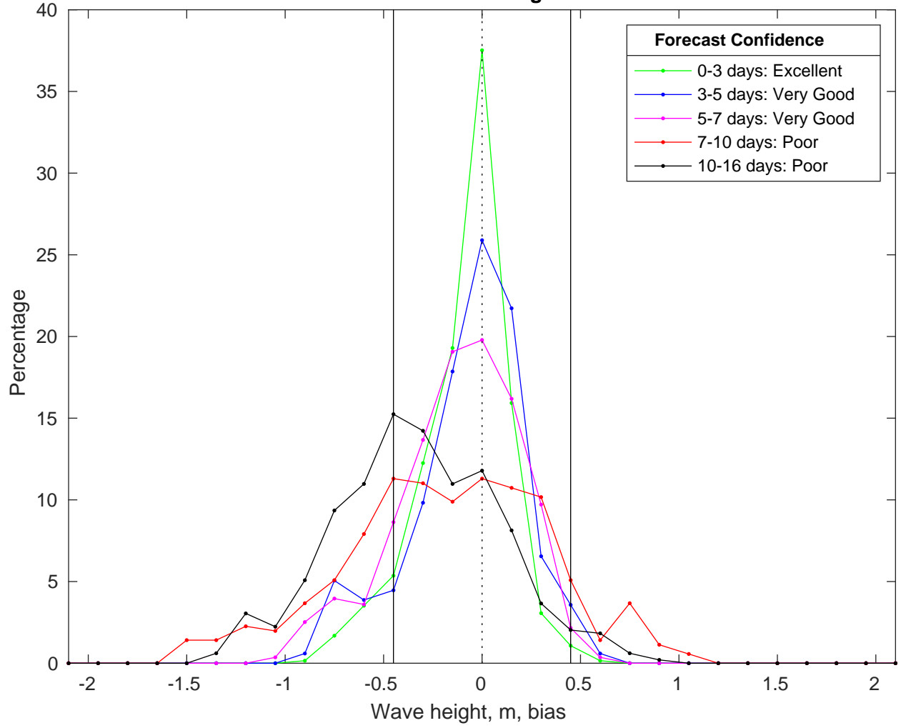
NDBC 42035 vs GFS Waves Bias Histogram: 24-Feb-2025
