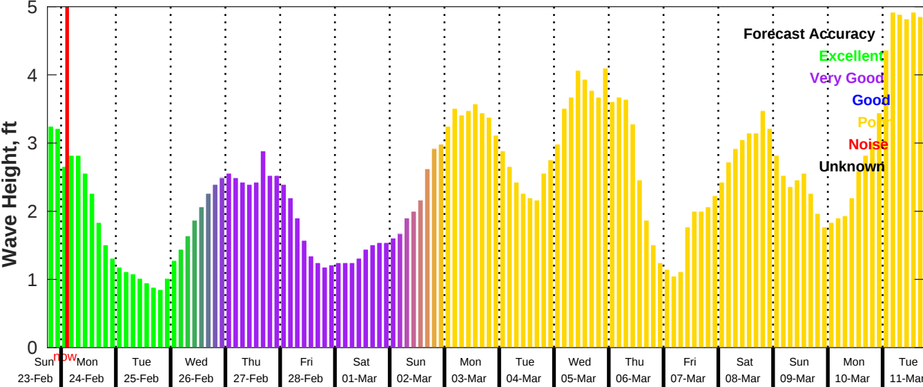
GFS Wave Forecast for NDBC 42035 from 23-Feb-2025 18:00:00 to 11-Mar-2025 18:00:00
