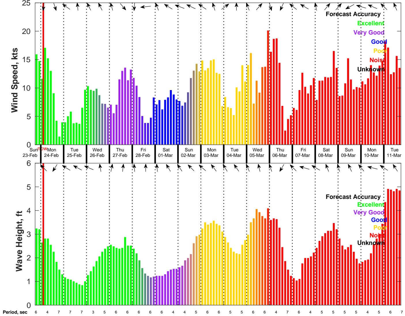
Wind & Wave Forecast for NDBC 42035 from 23-Feb-2025 18:00:00 to 11-Mar-2025 18:00:00
