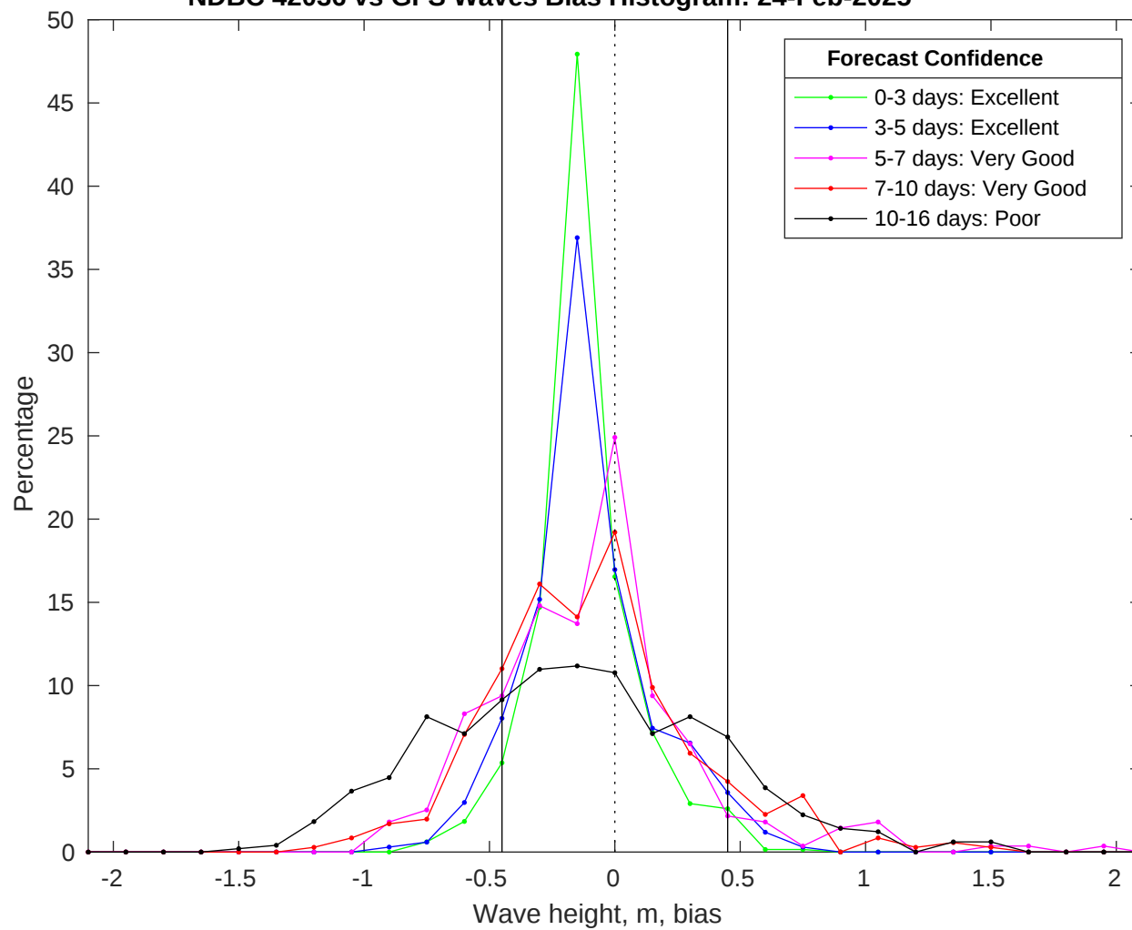
NDBC 42036 vs GFS Waves Bias Histogram: 24-Feb-2025
