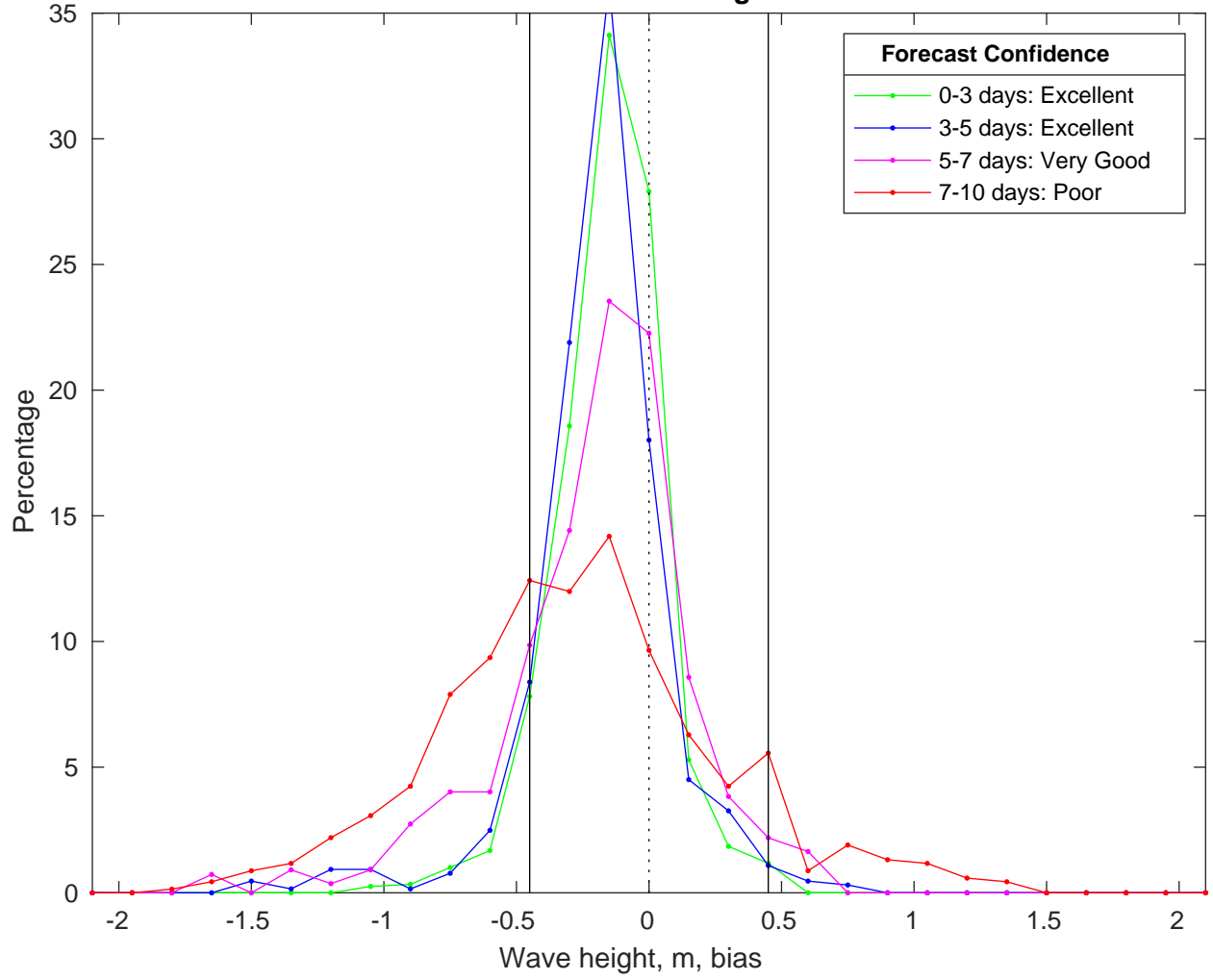
NDBC 42040 vs CMEMS Waves Bias Histogram: 24-Feb-2025
