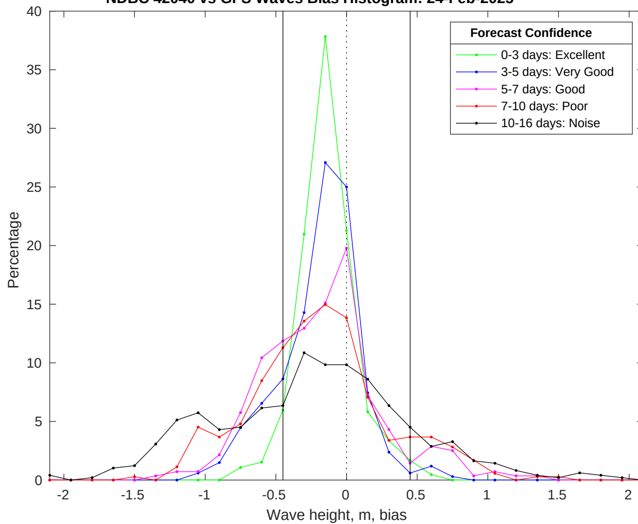
NDBC 42040 vs GFS Waves Bias Histogram: 24-Feb-2025
