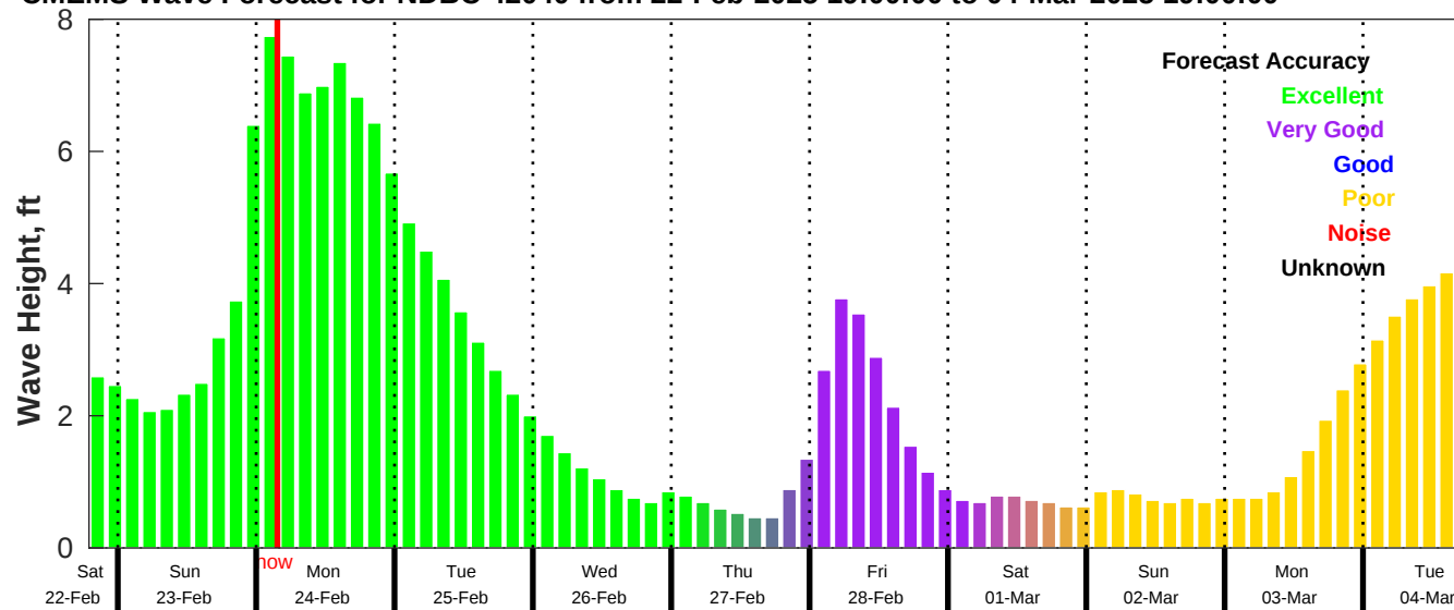
CMEMS Wave Forecast for NDBC 42040 from 22-Feb-2025 19:00:00 to 04-Mar-2025 19:00:00
