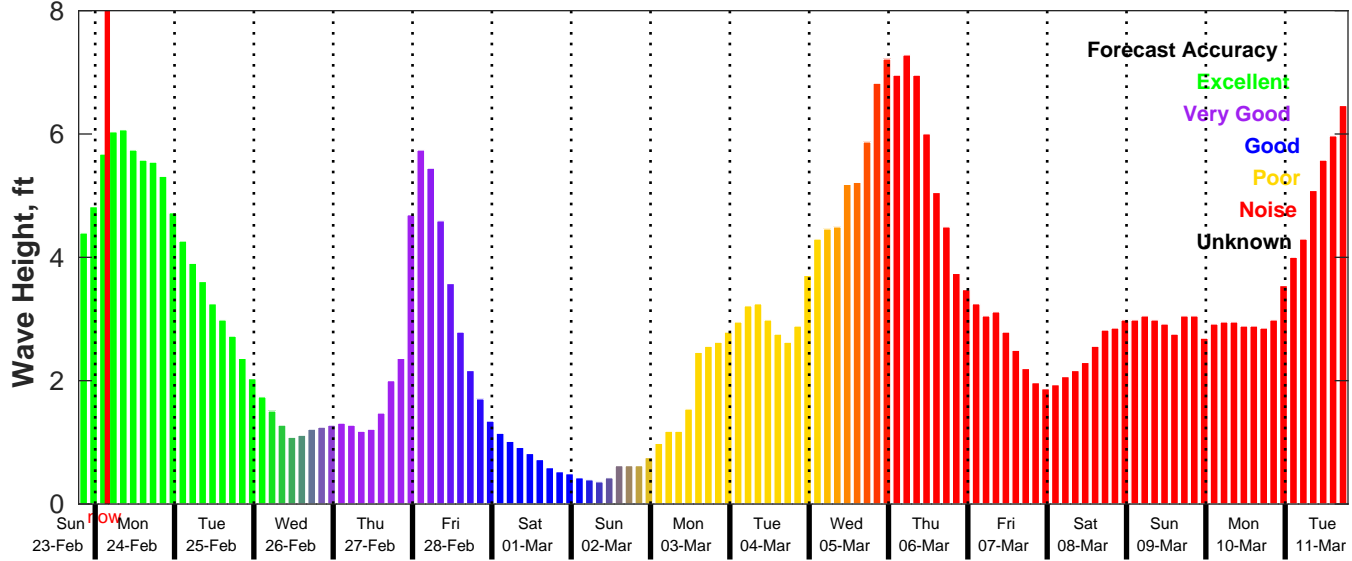
GFS Wave Forecast for NDBC 42040 from 23-Feb-2025 19:00:00 to 11-Mar-2025 19:00:00
