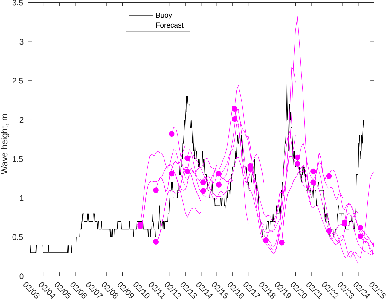
NDBC 42084 vs CMEMS Waves: 7 to 10 day forecast
