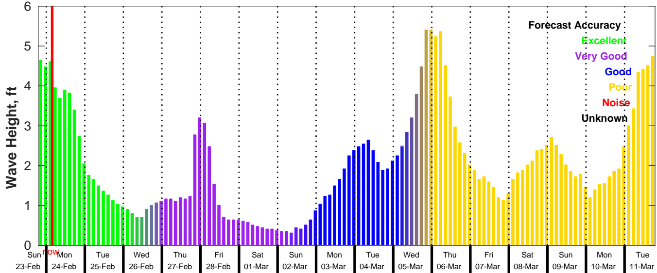
GFS Wave Forecast for NDBC 42084 from 23-Feb-2025 19:00:00 to 11-Mar-2025 19:00:00
