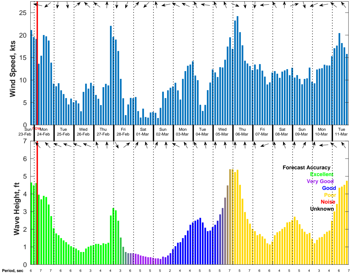
Wind & Wave Forecast for NDBC 42084 from 23-Feb-2025 19:00:00 to 11-Mar-2025 19:00:00
