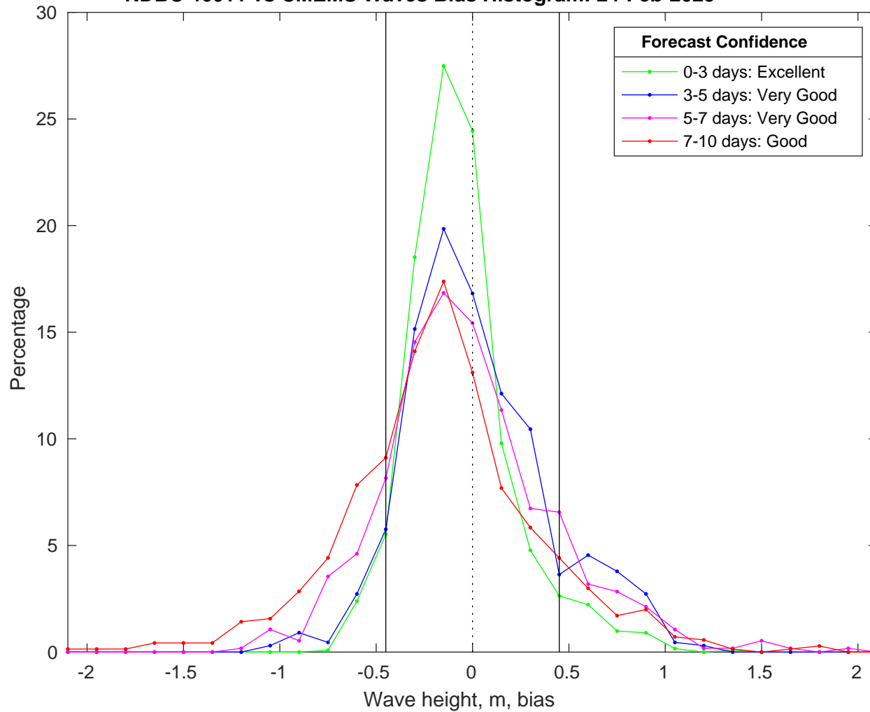
NDBC 46011 vs CMEMS Waves Bias Histogram: 24-Feb-2025
