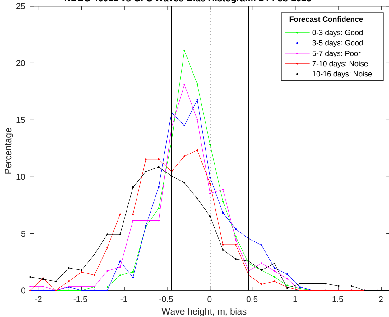
NDBC 46011 vs GFS Waves Bias Histogram: 24-Feb-2025
