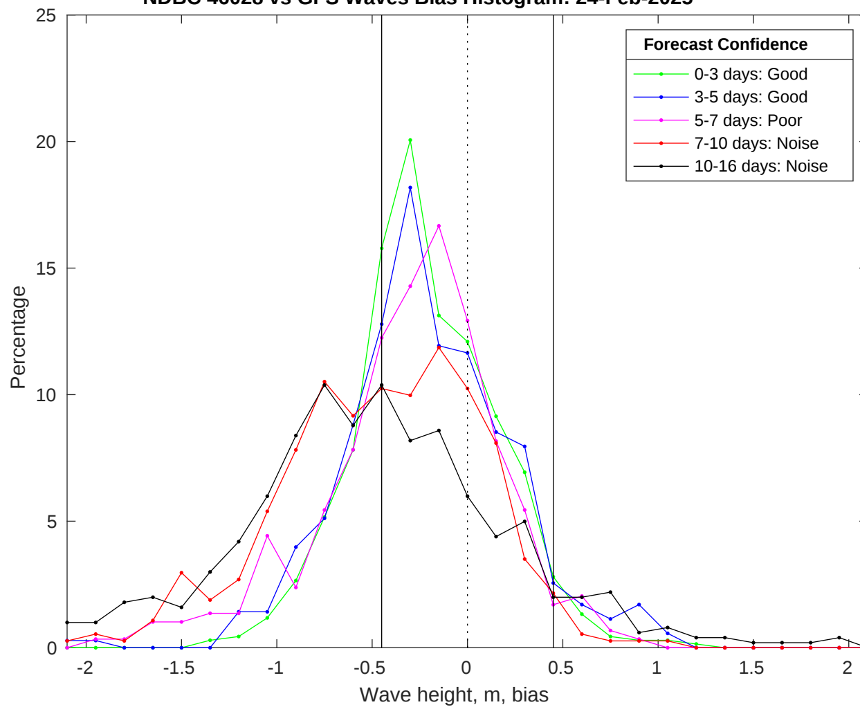
NDBC 46028 vs GFS Waves Bias Histogram: 24-Feb-2025
